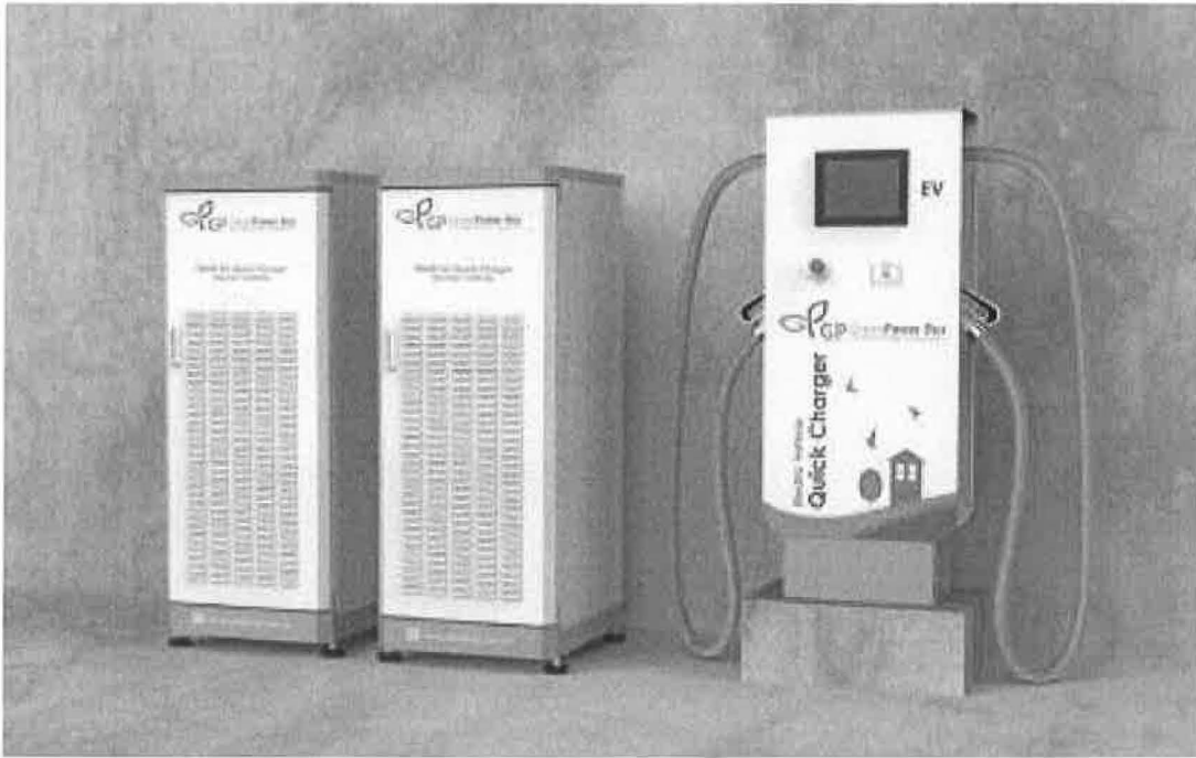
Figure 4 – GreenPower Charging Station Power Supply and Pedestal
