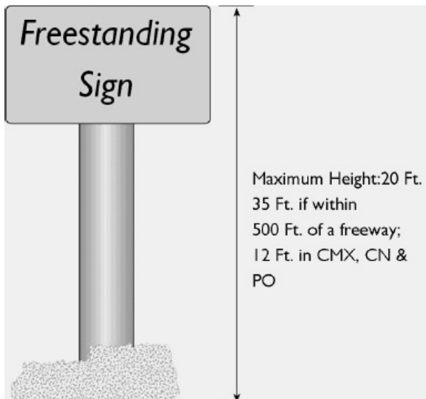
FIGURE 305.10G: FREESTANDING SIGNS
